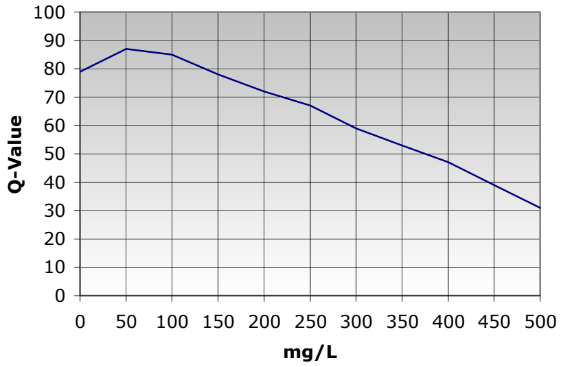
Chart 7 Total Dissolved Solids
