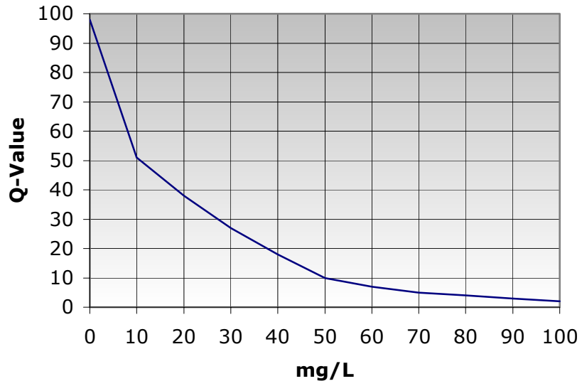
Chart 4 Nitrate Results
